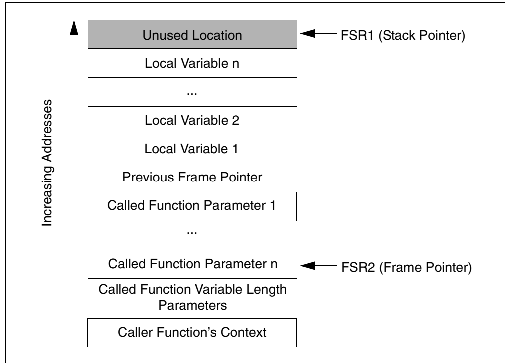
FIGURE 3-4: EXAMPLE OF SOFTWARE STACK IMMEDIATELY FOLLOWING A C FUNCTION CALL IN EXTENDED MODE
